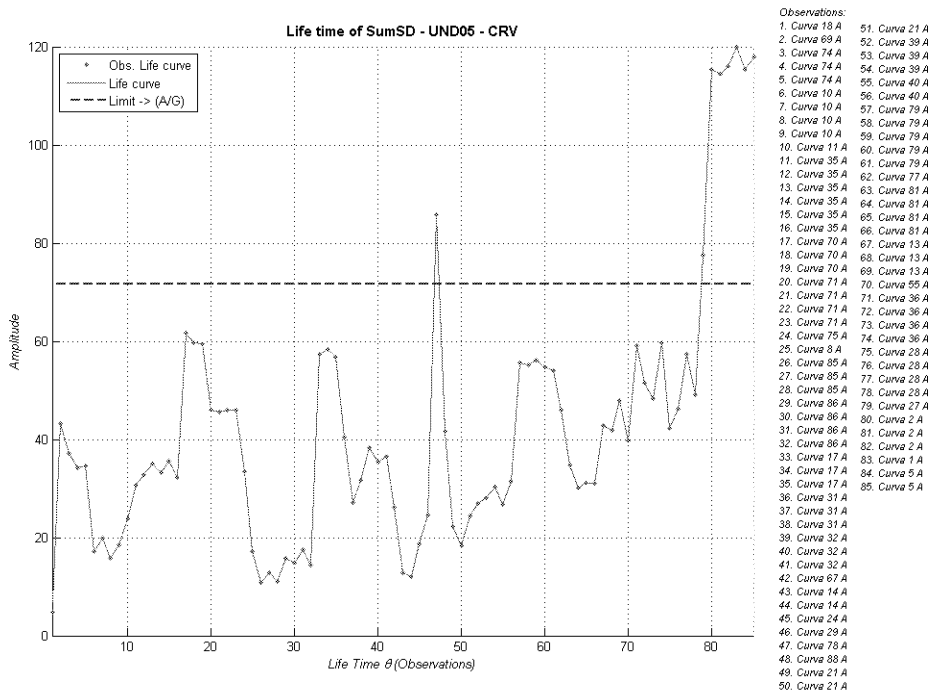
Fig.3: Profile of the general failure
