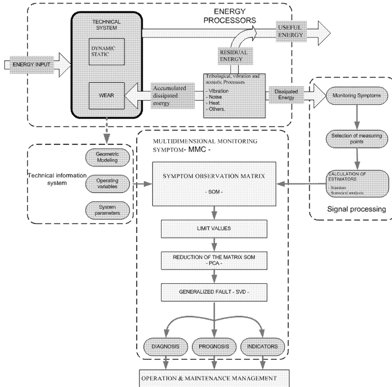
Fig.2: Methodology for a holistic approximation
