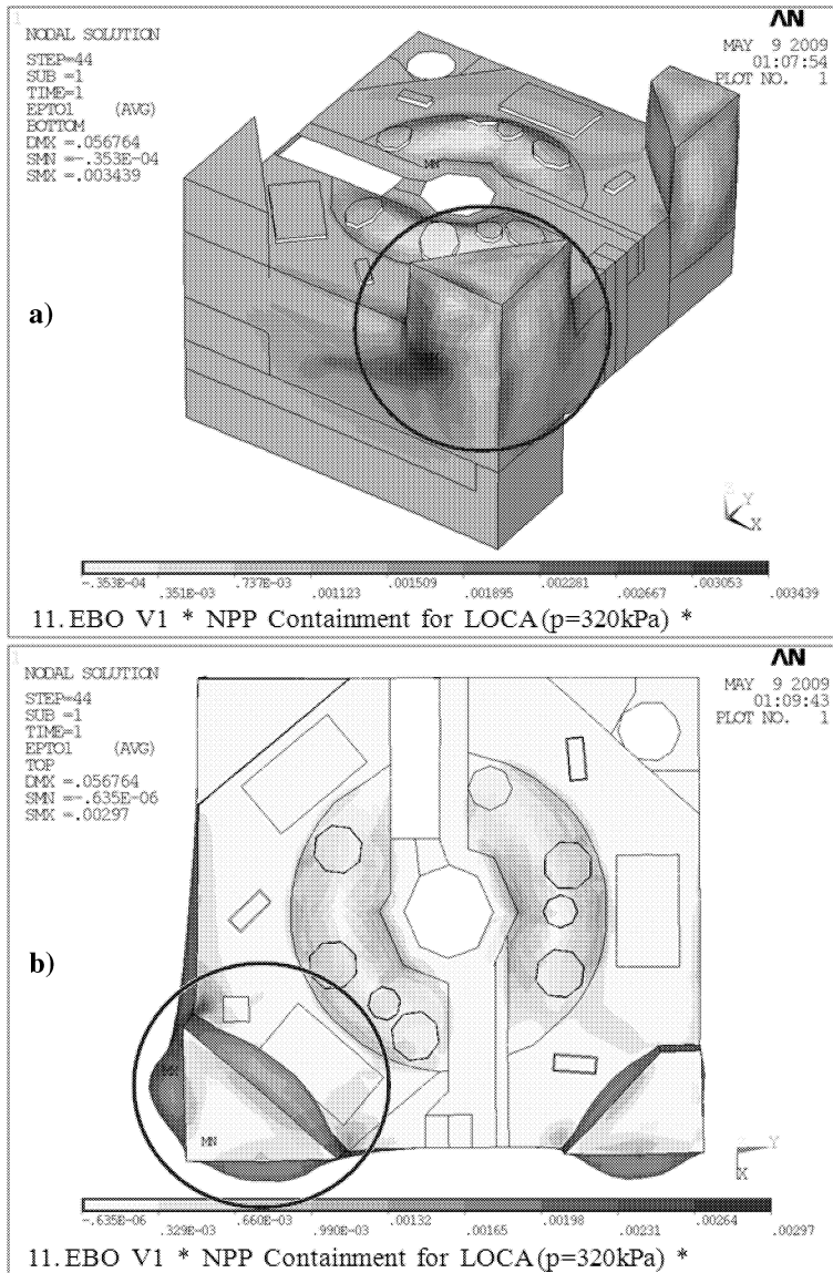
Fig.10: Critical area of containment structure loading at overpressure 320 kPa
