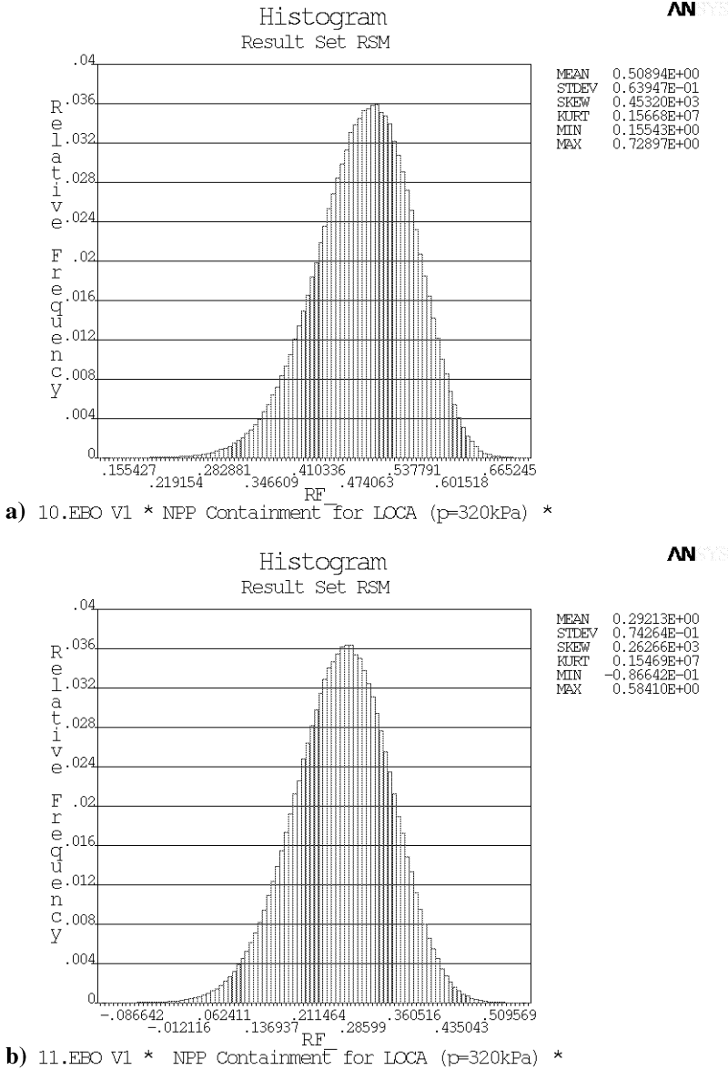
Fig.15: Reliability function RF under overpressure 320 kPa for two models: a) without the degradation effect, b) with the degradation effect
