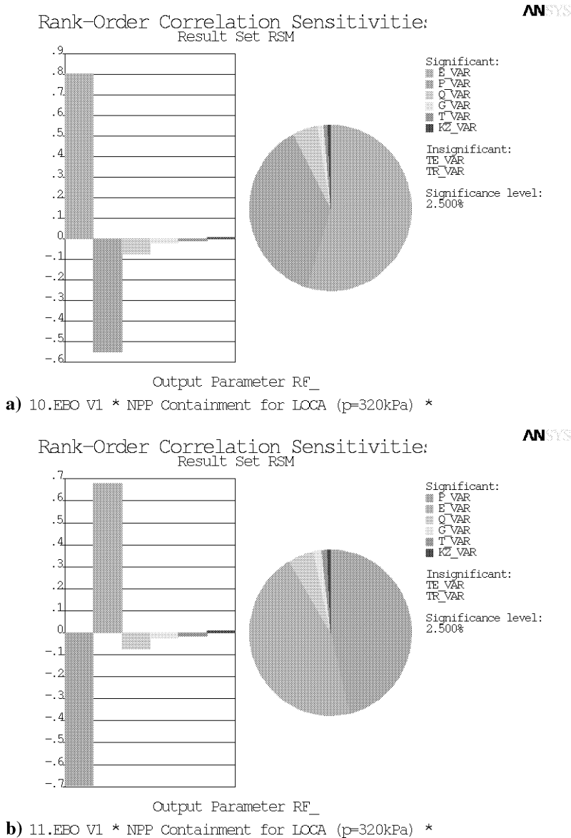
Fig.14: Sensitivity of reliability function RF
