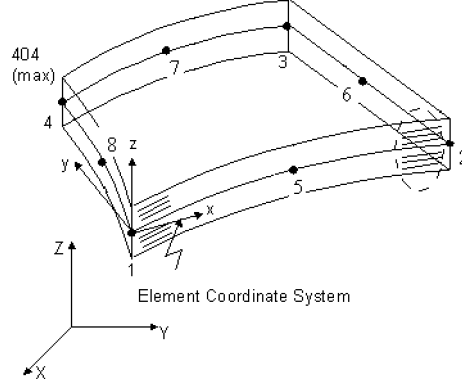
Fig.3: The shell element with 8 nodes
